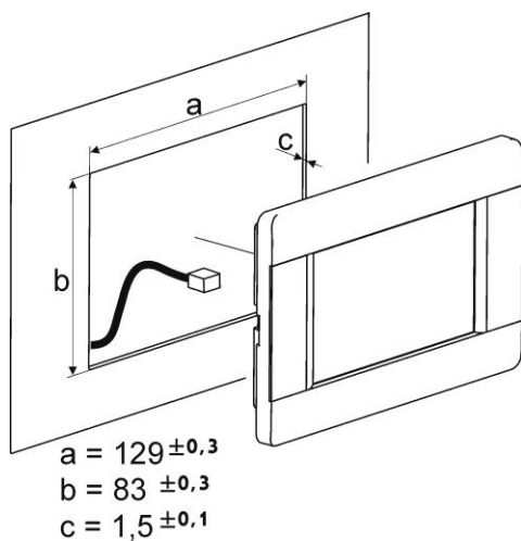
Obr. 17 Montáž panelu ecoSTER TOUCH.
